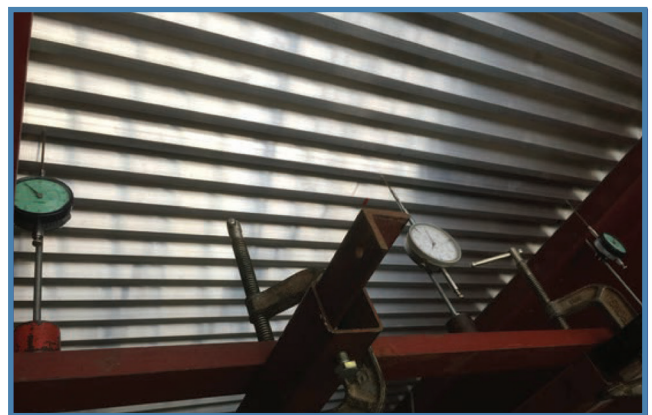
Internal View of Horizontal line load test
