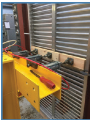
Horizontal Line Load (Internal view of test)
